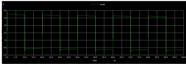
Figure 4.12: Simulation output of LM3411
