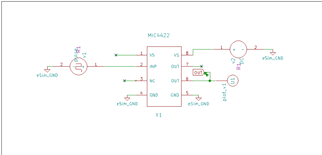
Figure 4.31: Test bench circuit of MIC4422
