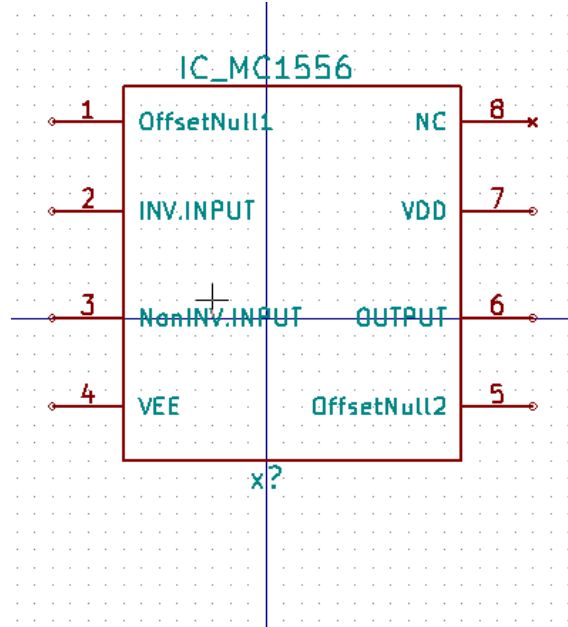
Figure 4.13: Schematic symbol of MC1556
