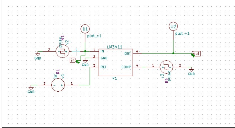
Figure 4.11: Test bench circuit of LM3411
