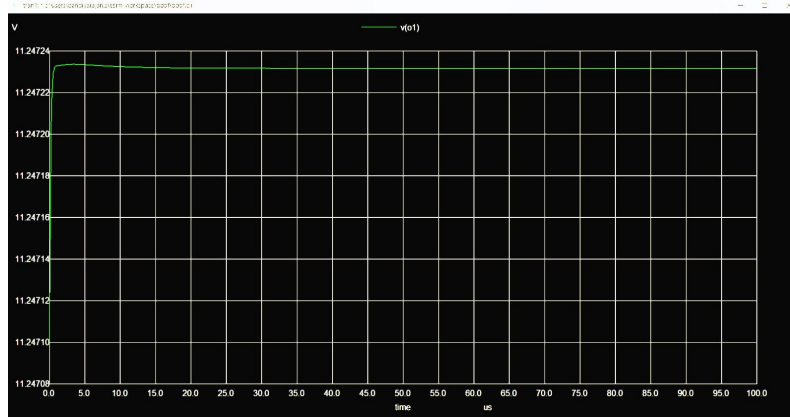
Figure 4.24: Simulation output of TL317
