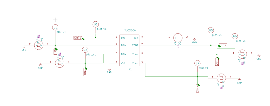
Figure 4.3: Test bench circuit of TLC2264
