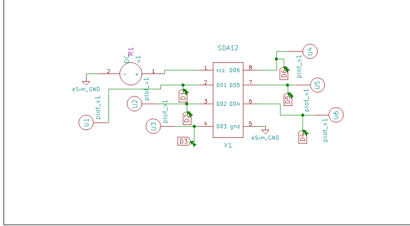
Figure 4.19: Test bench circuit of SDA12
