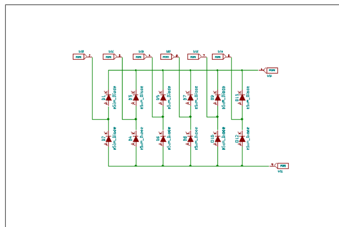
Figure 4.18: Subcircuit schematic of SDA12
