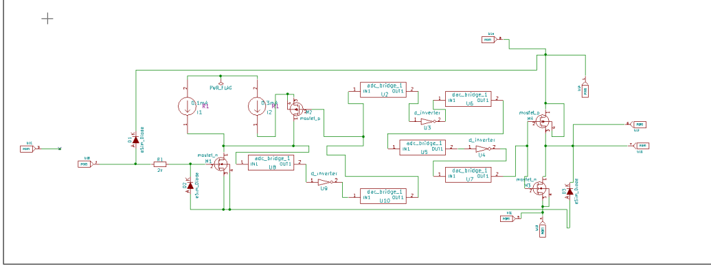
Figure 4.30: Subcircuit schematic of MIC4422
