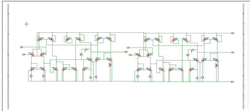
Figure 4.2: Subcircuit schematic of TLC2264
