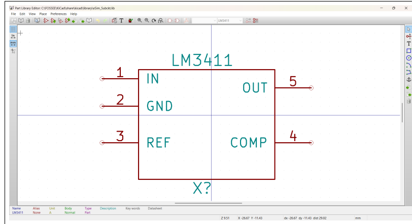
Figure 4.9: Schematic symbol of LM3411
