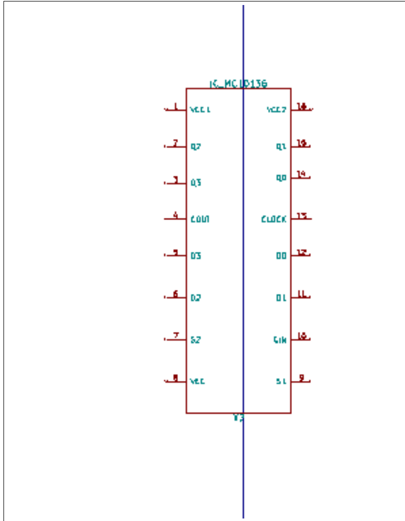
Figure 4.37: Schematic symbol of MC10136
