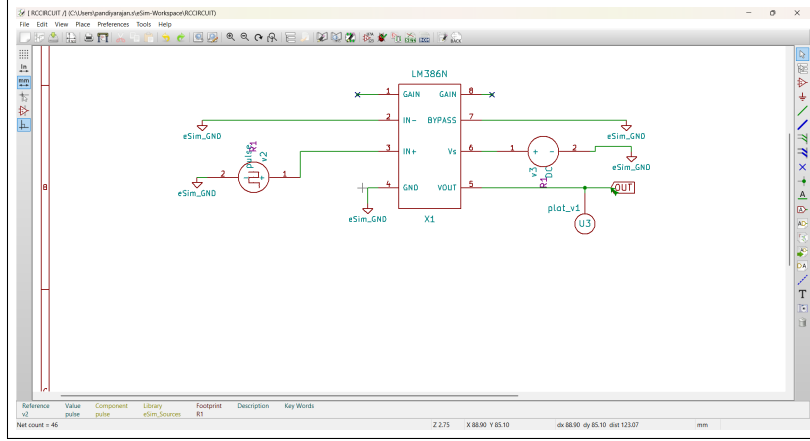
Figure 4.7: Test bench circuit of LM386N
