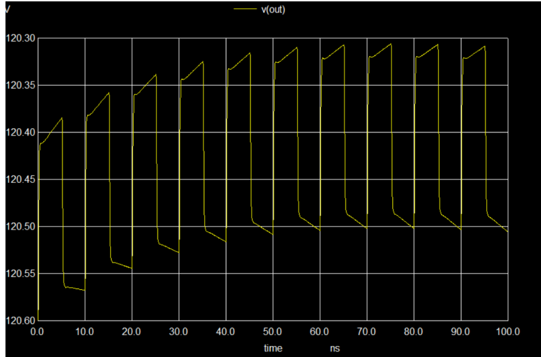
Figure 4.8: Simulation output of LM386N
