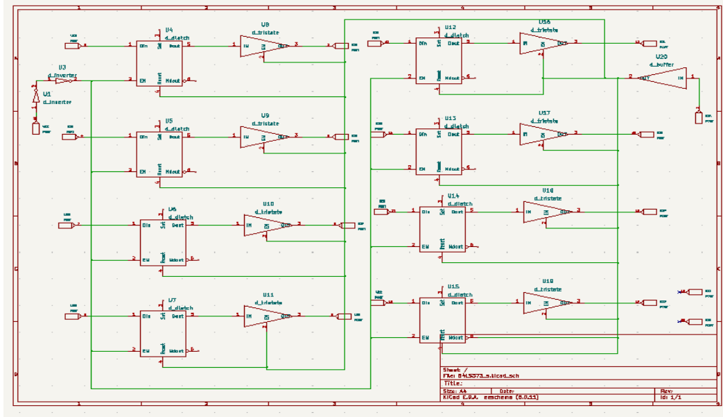
Figure 4.2: Subcircuit Schematic of SN54LS373
