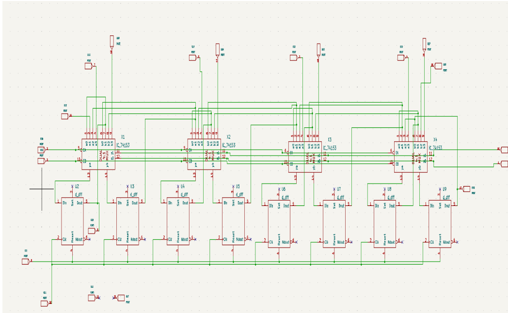
Figure 4.17: Subcircuit Schematic of SN74LS299
