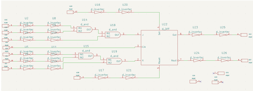
Figure 5.3: Subcircuit Schematic diagram of the CD4095 IC
