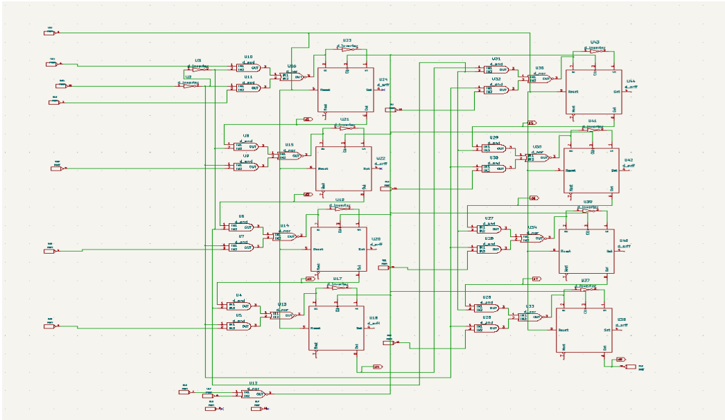
Figure 4.7: Subcircuit Schematic of SN54166
