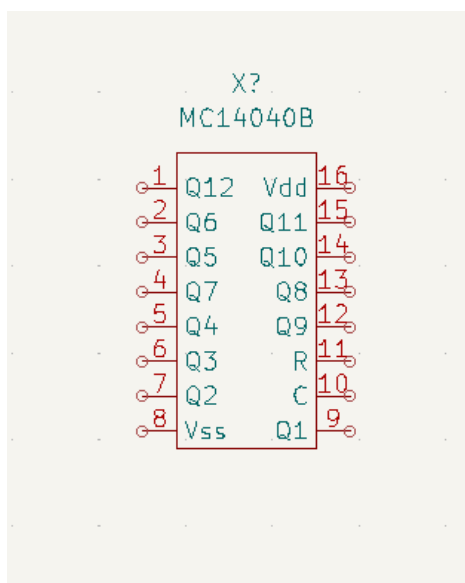
Figure 4.51: Pin diagram of MC14040B
