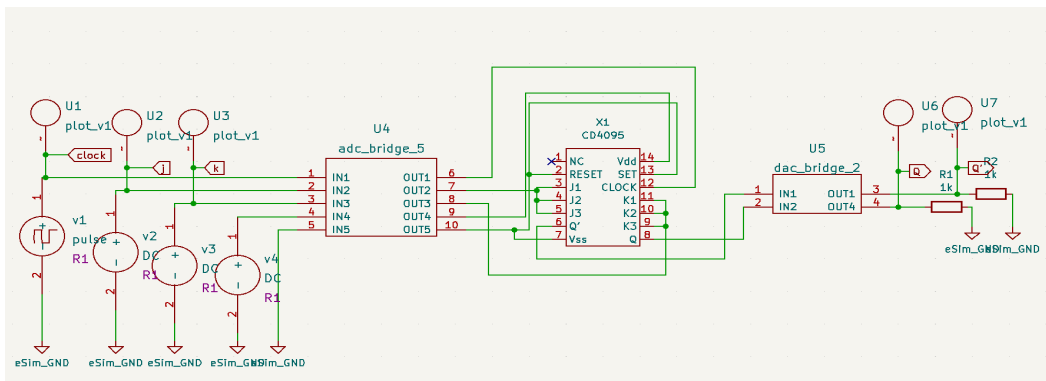
Figure 5.4: Test Circuit of the CD4095 IC
