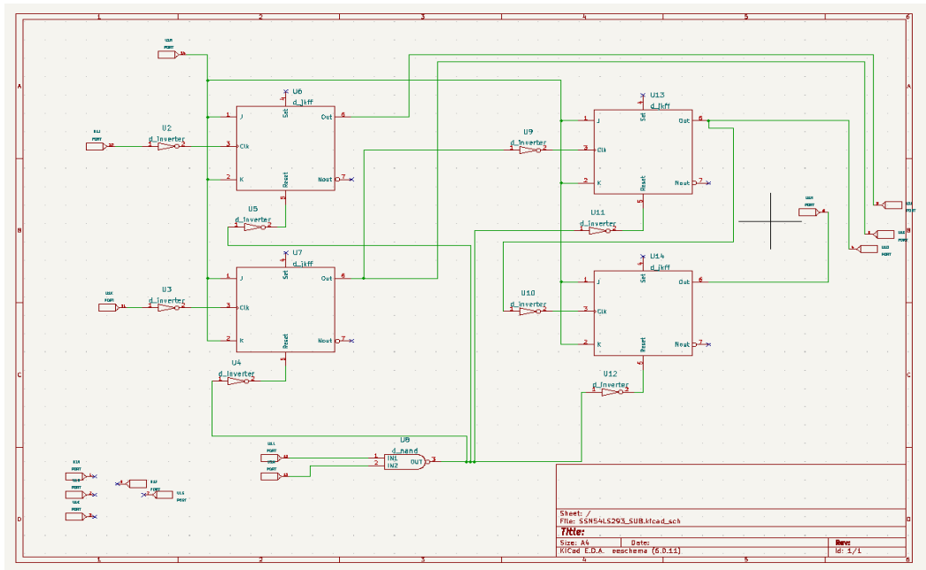
Figure 4.27: Subcircuit Schematic of SN54LS293
